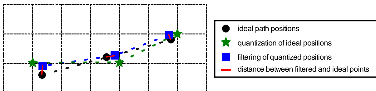
Figure 8. Illustration of the quantization and Kalman filter process conducted over an ideal sample trajectory. The RMSE is defined, according Equation (13), as the square root of the average of all the distances squared with respect to the real reference path position.
