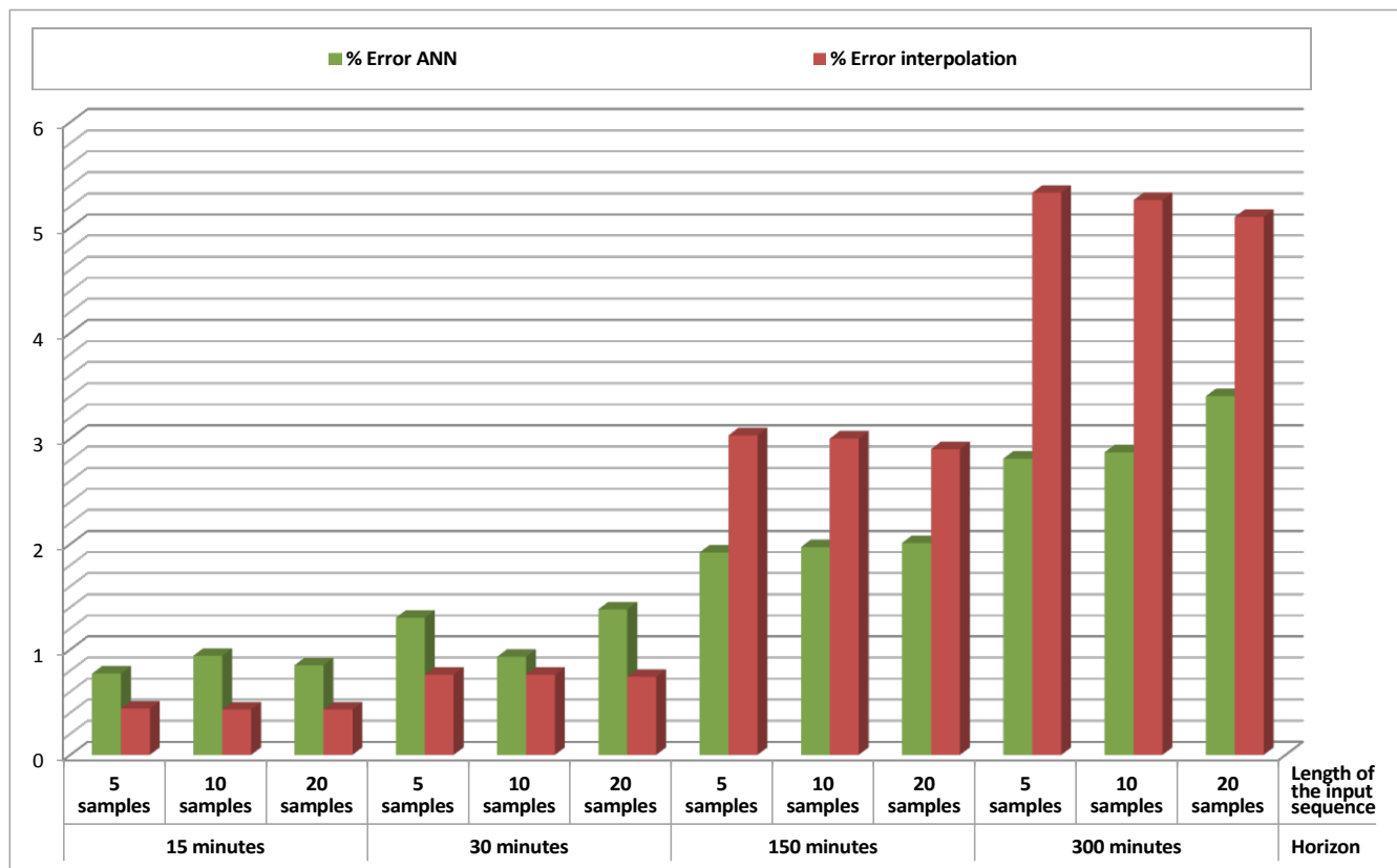
Figure 8. Data prediction results (% error ANN/% error interpolation) for temperature in Sensor 1, using temperature in Sensor 1 as an input.
